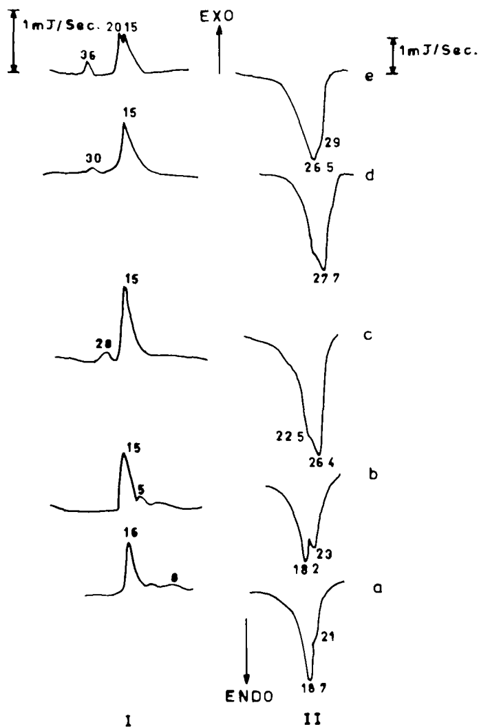
FIG. 2. I, DSC cooling curves at the rate of 2^{\circ}\text{C}/\text{min} . II, DSC, heating curves ( 10^{\circ}\text{C}/\text{min} ) after cooling at 2^{\circ}\text{C}/\text{min} . a, b, c, d, and e, respectively, indicate the curves of TG and TG containing DHS-TG at 2, 5, 8 and 10%.
