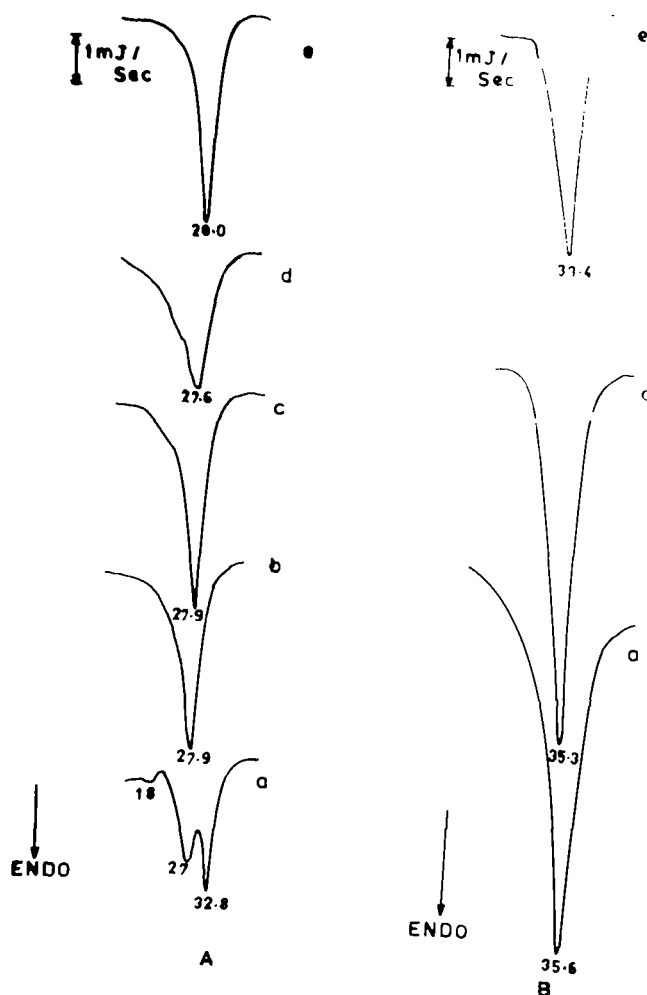
FIG. 3. A, DSC heating curves ( 10^{\circ}\text{C}/\text{min} ) of samples tempered at 0^{\circ}\text{C} for 18 hr. B, DSC heating curves ( 10^{\circ}\text{C}/\text{min} ) of samples tempered at 0^{\circ}\text{C} for one hr and at 26^{\circ}\text{C} for 3 hr. a, b, c, d, e, respectively, indicate the curves of TG and TG containing DHS-TG at 2, 5, 8 and 10% levels.
